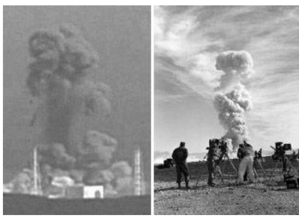
Figure 773: The explosion at Fukushima compared with the cloud produced by a small nuclear weapon.
