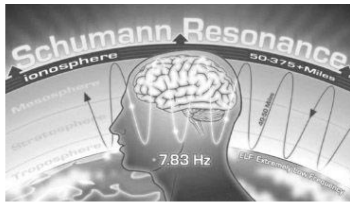
Figure 768: The realm of Schumann Cavity Resonance.
