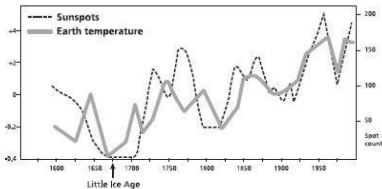
Figure 673: Earth temperature and sunspots. The lowest point of sunspot activity, known as the Maunder Minimum, brought the Little Ice Age.
