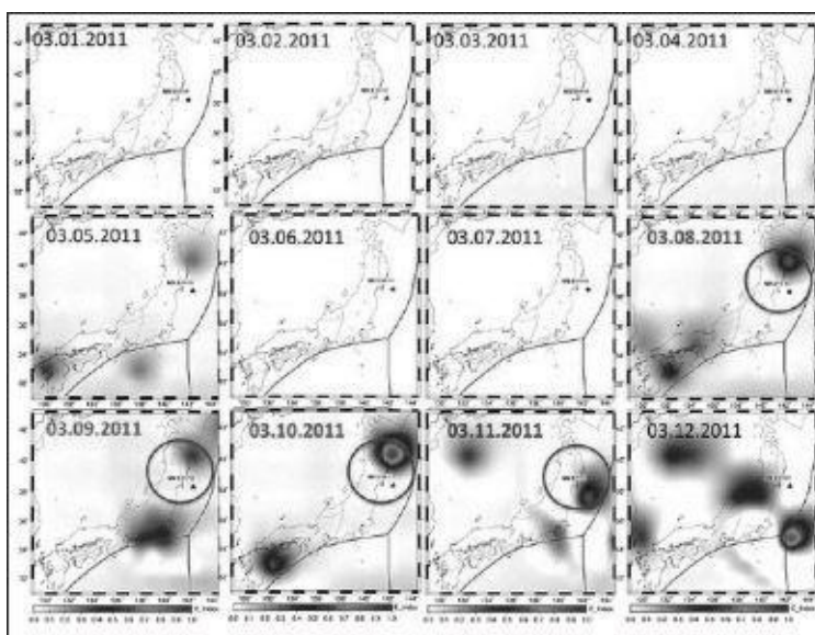
Figure 756: Infrared emissions above the quake epicentre in Japan increased dramatically in the days leading up to the disaster.
