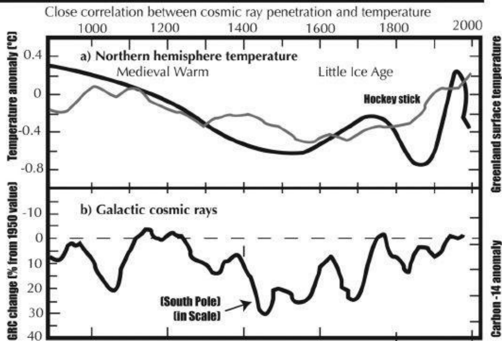
Figure 669: The CERN findings confirm the bloody obvious – the clear connection between cosmic rays and Earth temperature.
