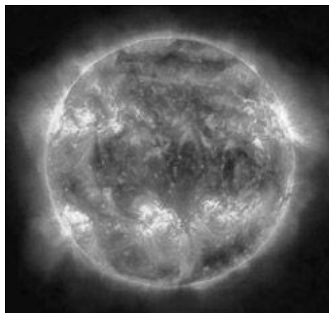
Figure 668: Anyone think that the Sun might affect the temperature?
